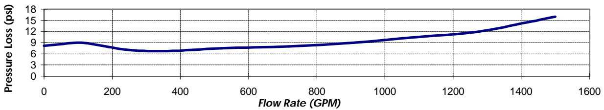
■ 8" Documented Flow Characteristics
