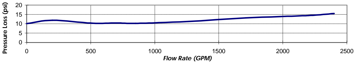
■ 10" Documented Flow Characteristics
