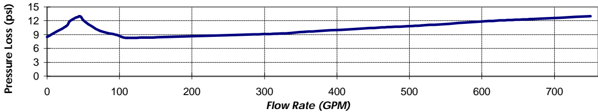
■ 6" Documented Flow Characteristics
