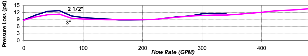
■ 4" Documented Flow Characteristics
