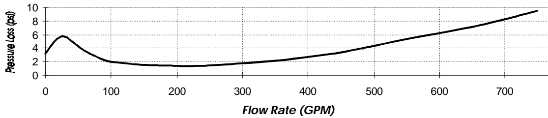
■ 6" Documented Flow Characteristics
