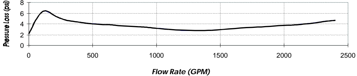
■ 10" Documented Flow Characteristics
