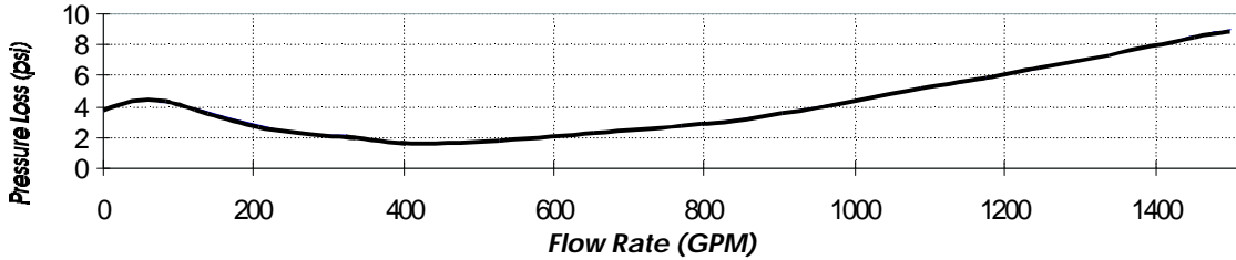
■ 6" Documented Flow Characteristics
